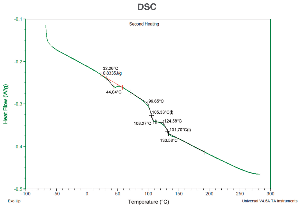
Figure 1. 2nd heating scan DSC data for the PC-ABS Flat (XY) sample.
